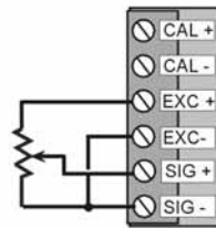
3-Wire Transducer
