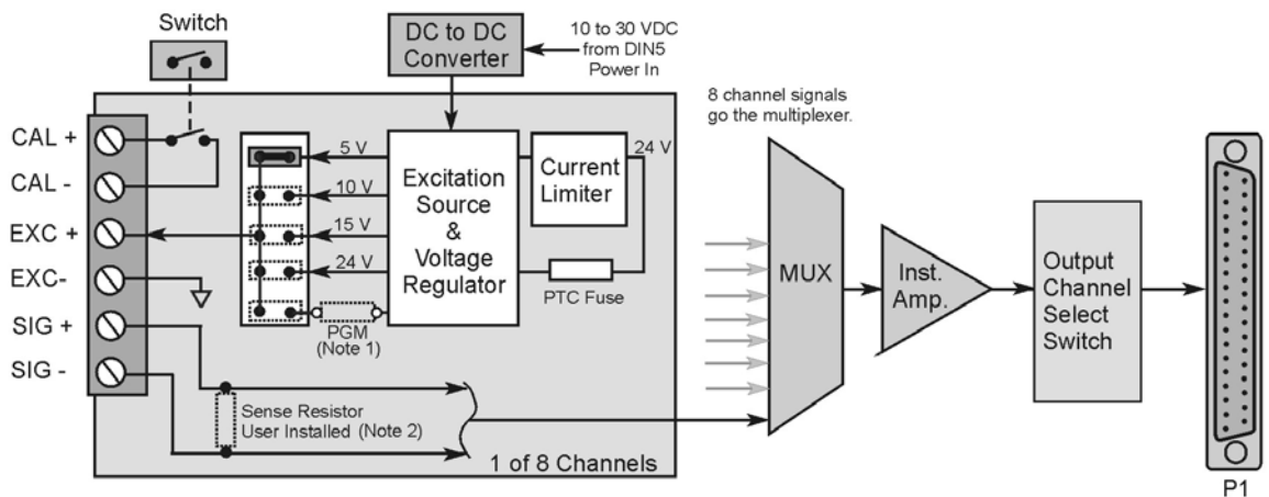
DBK65 Block Diagram
