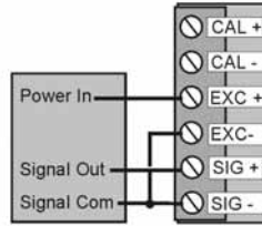
3-Wire Transducer
