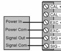
4-Wire Transducer
