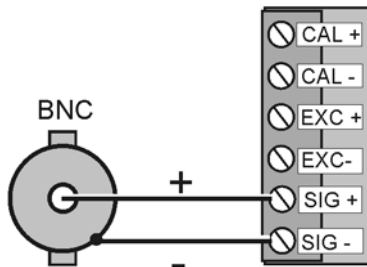
Connecting a BNC to SIG+ and SIG-
