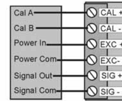
4-Wire Transducer with internal calibration
