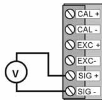
2-Wire Volts
