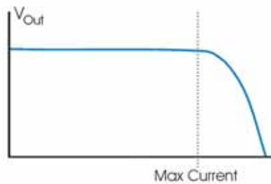
Typical Current Limiting Voltage Curve
