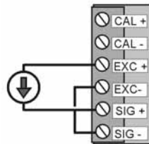
2-Wire Transducer with 4 to 20 mA output
