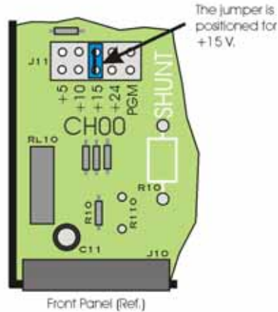
Reference for Selecting a Pre-Set Voltage Value
